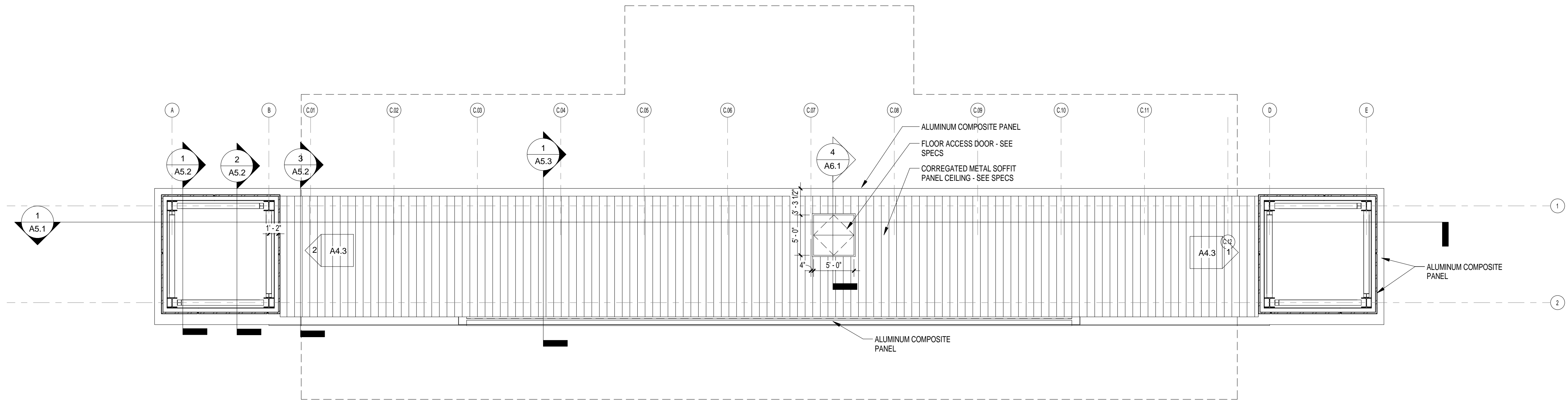
1 PLAN @ UNDERSIDE OF CATWALK 1 A2.1 1/8" = 1'-0" REFERENCED ON:
