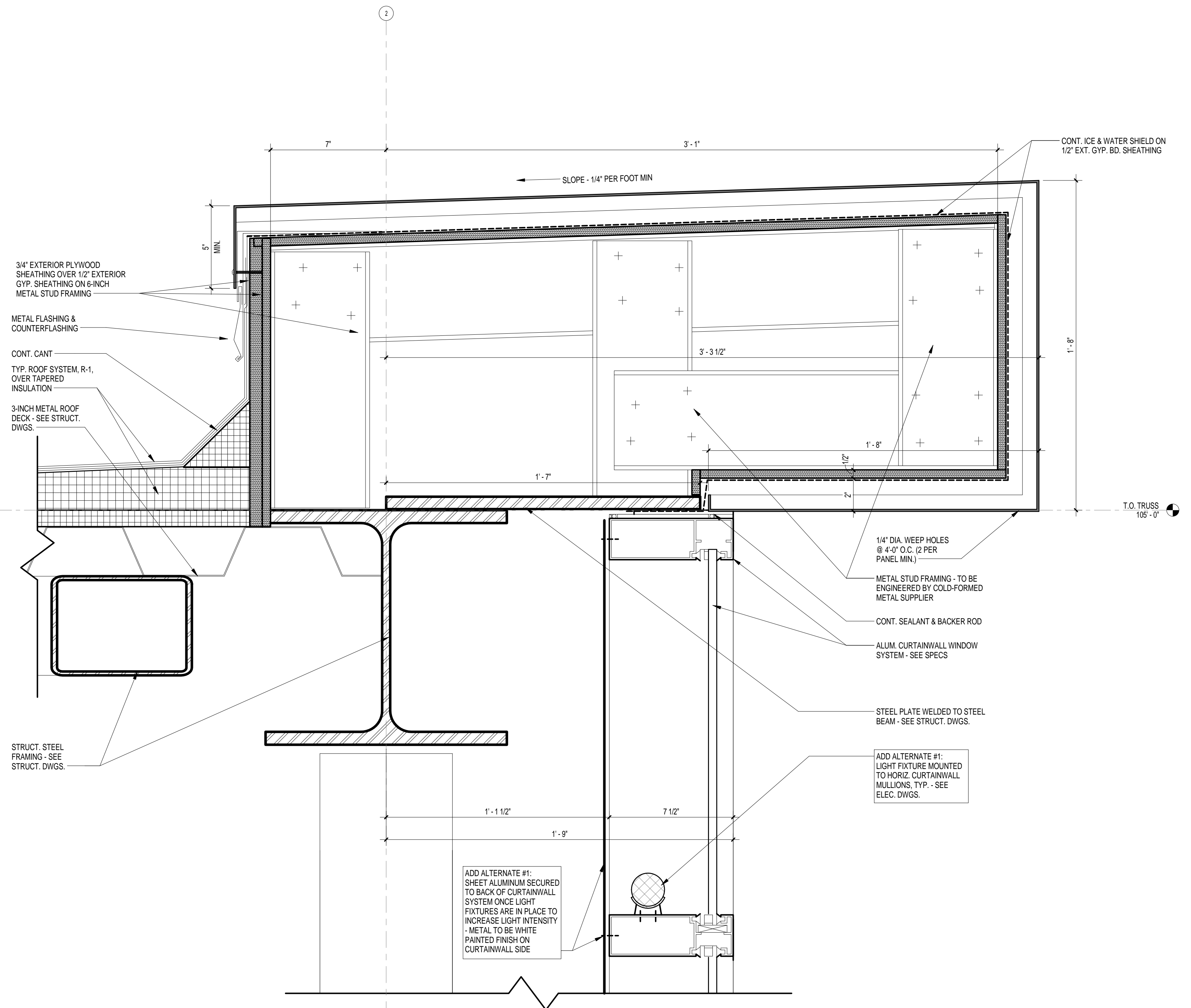
1 HEAD SECTION DETAIL A7.2 3" = 1'-0" REFERENCED ON: A5.2
