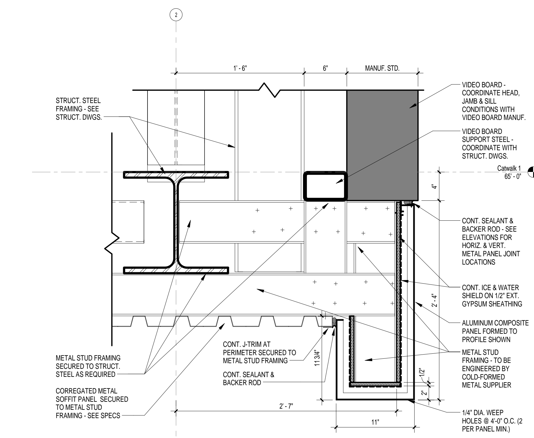
5 SECTION DETAIL A5.3 1 1/2" = 1'-0" REFERENCED ON: A5.2
