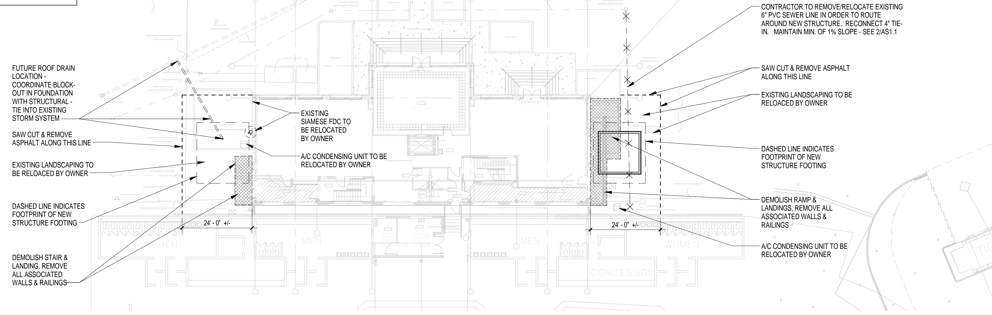
1 SITE DEMOLITION PLAN AS1.1 1" = 20'-0" REFERENCED ON:
