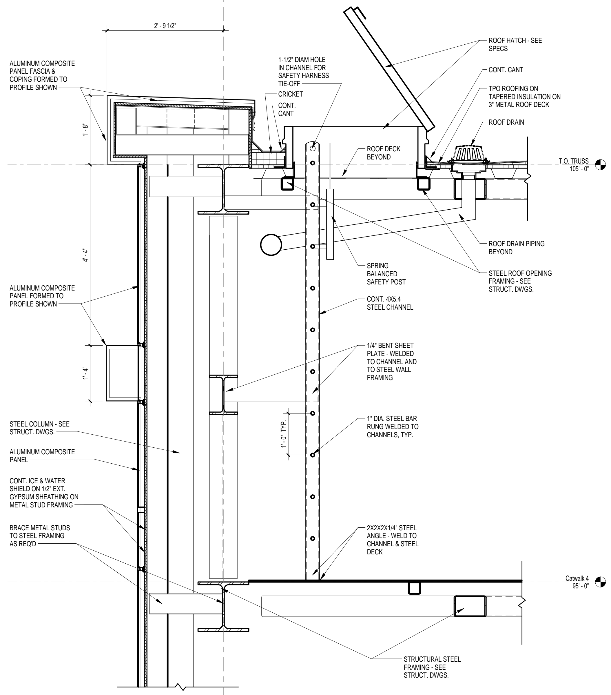
5 ROOF HATCH/ACCESS LADDER SECTION A6.1 3/4" = 1'-0" REFERENCED ON: A1.2
