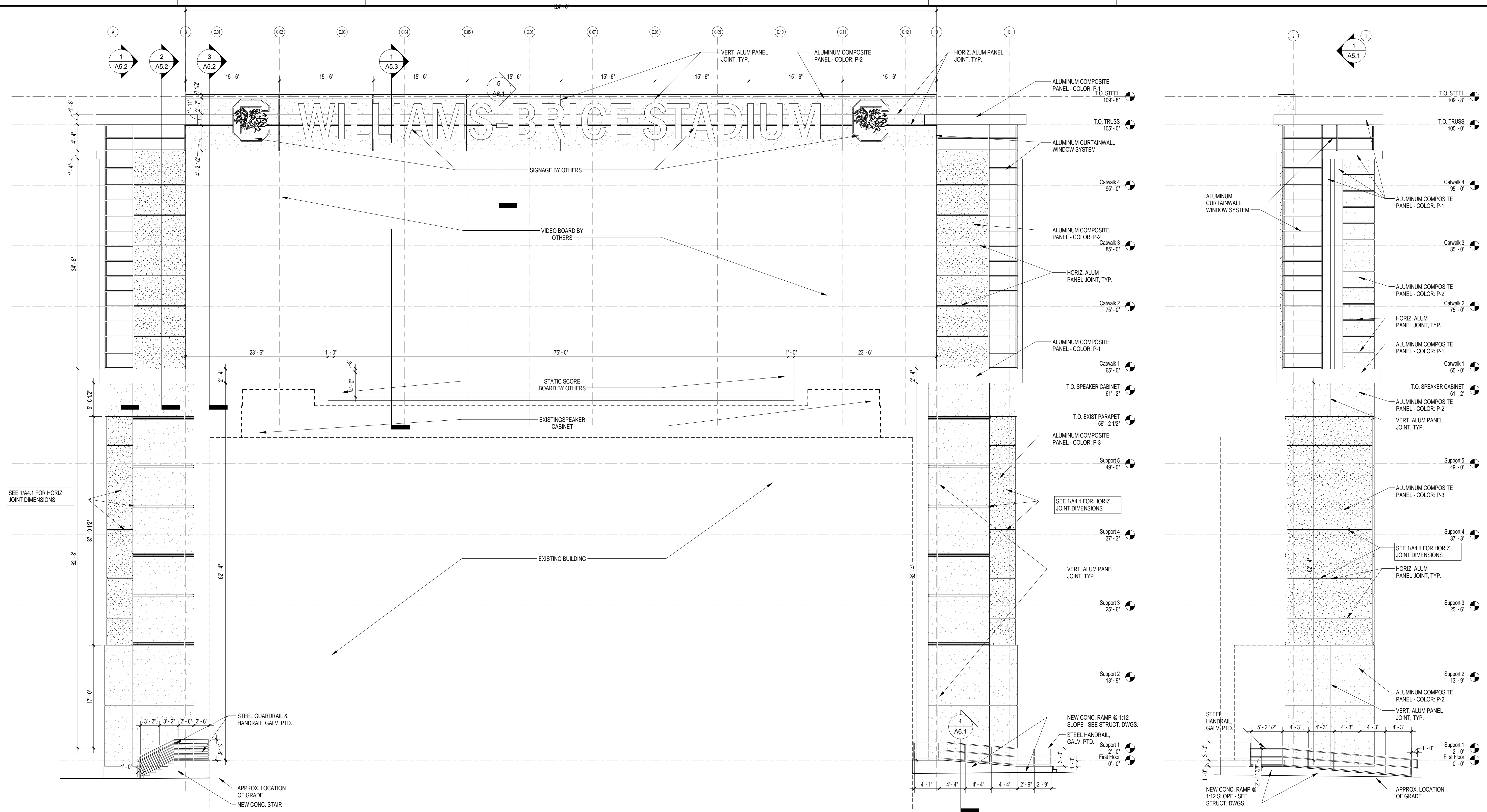
1 SOUTH ELEVATION A4.2 1/8" = 1'-0" REFERENCED ON: A1.1
