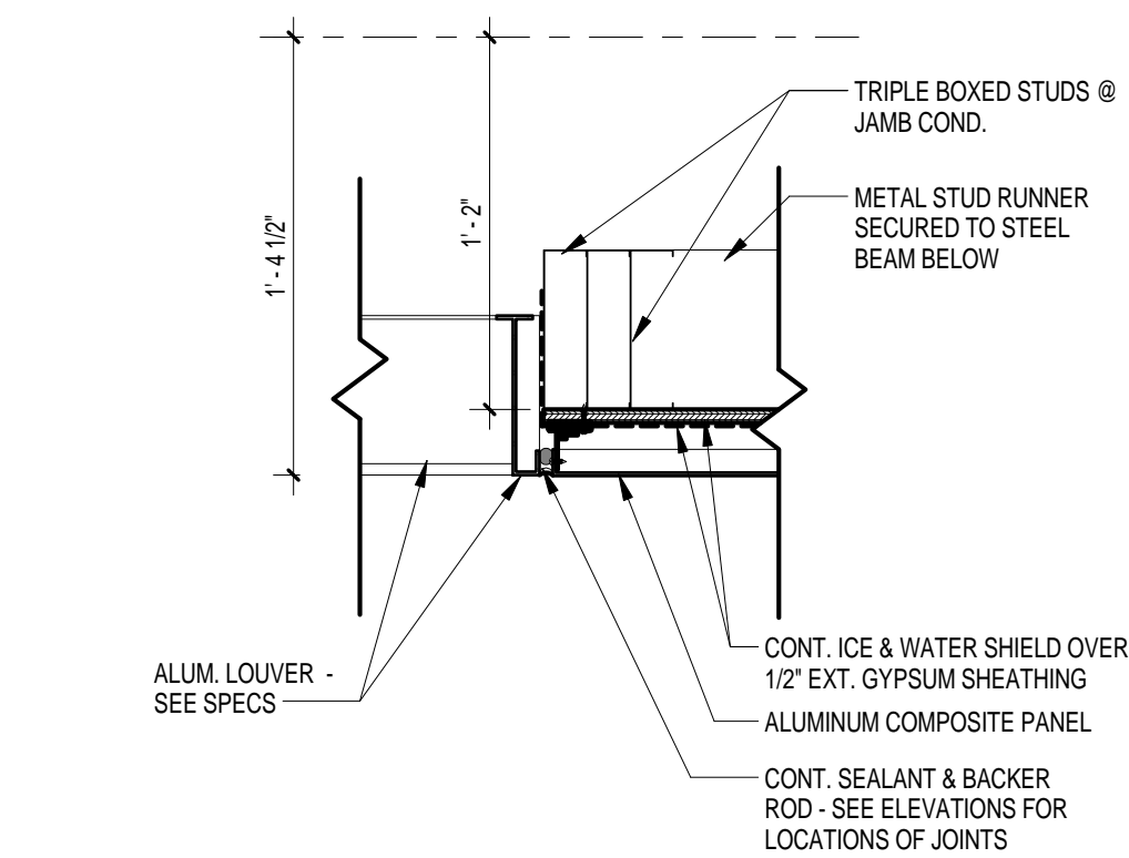
7 LOUVER JAMB PLAN DETAIL A4.3 1 1/2" = 1'-0" REFERENCED ON: A4.3
