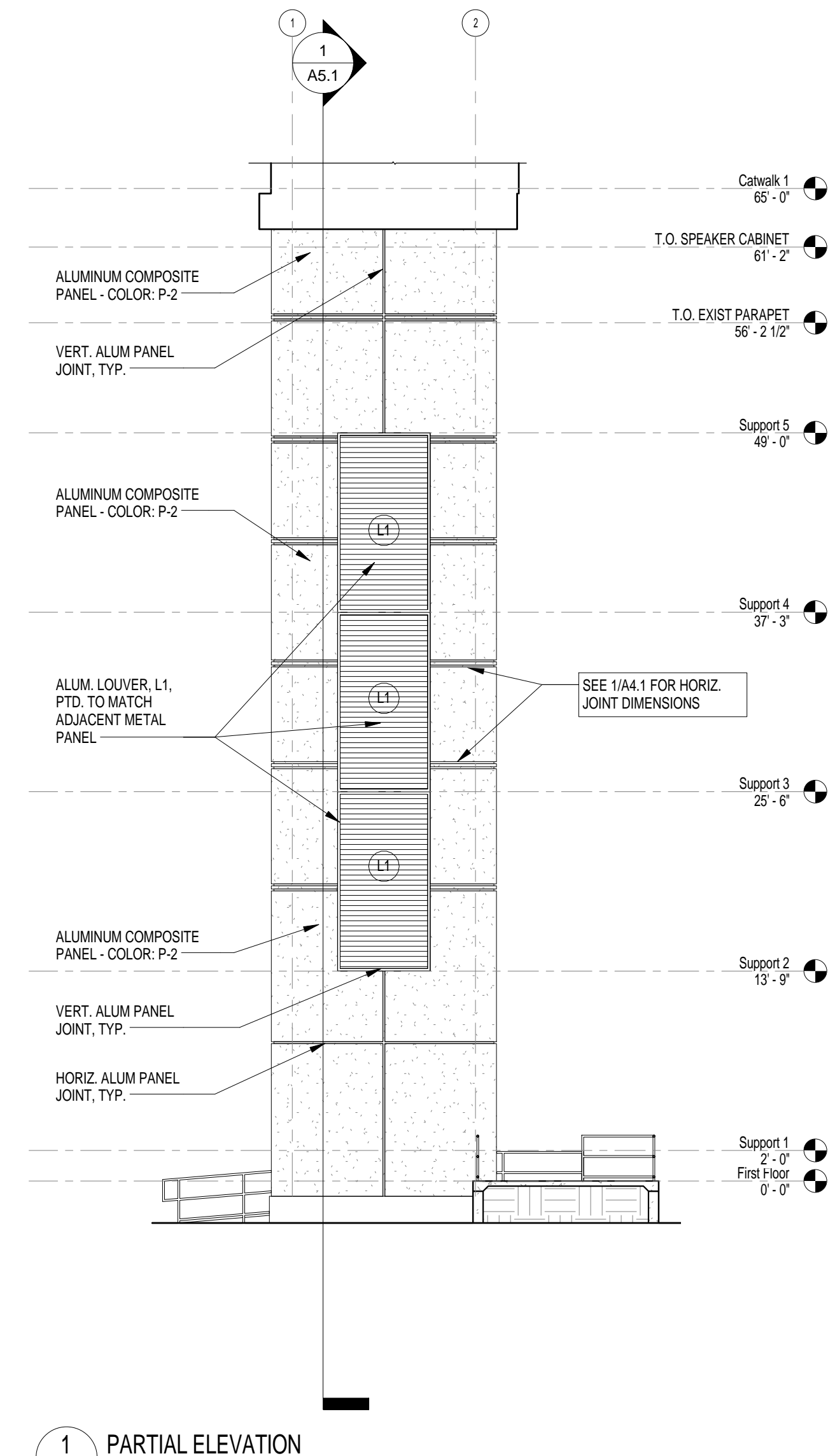
1 PARTIAL ELEVATION A4.3 1/8" = 1'-0" REFERENCED ON: A1.1
