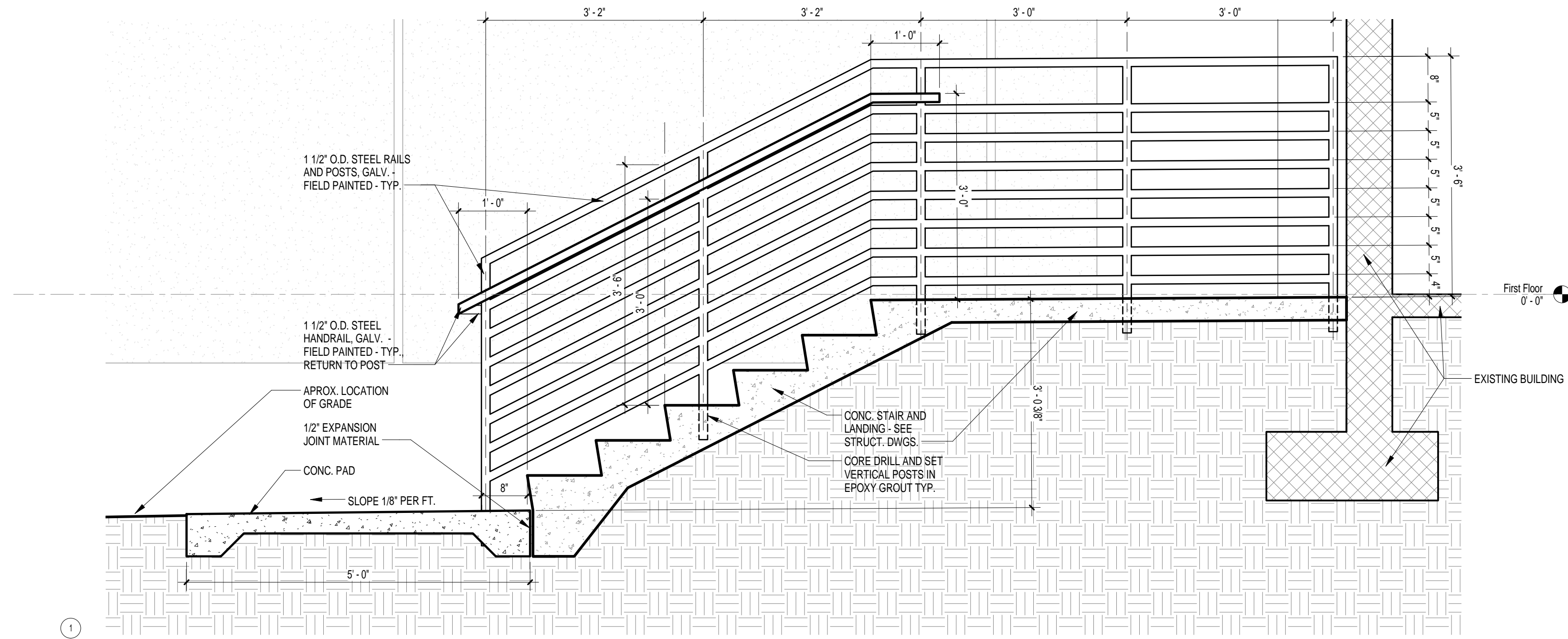
2 STAIR SECTION A6.1 3/4" = 1'-0" REFERENCED ON: A1.1
