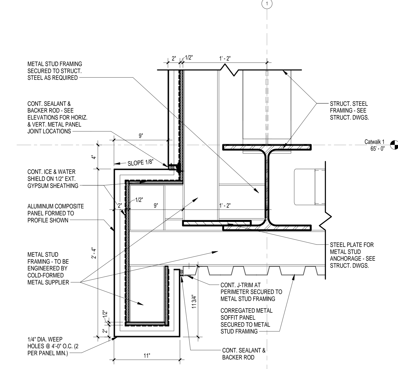
4 SECTION DETAIL A5.3 1 1/2" = 1'-0" REFERENCED ON: A5.2
