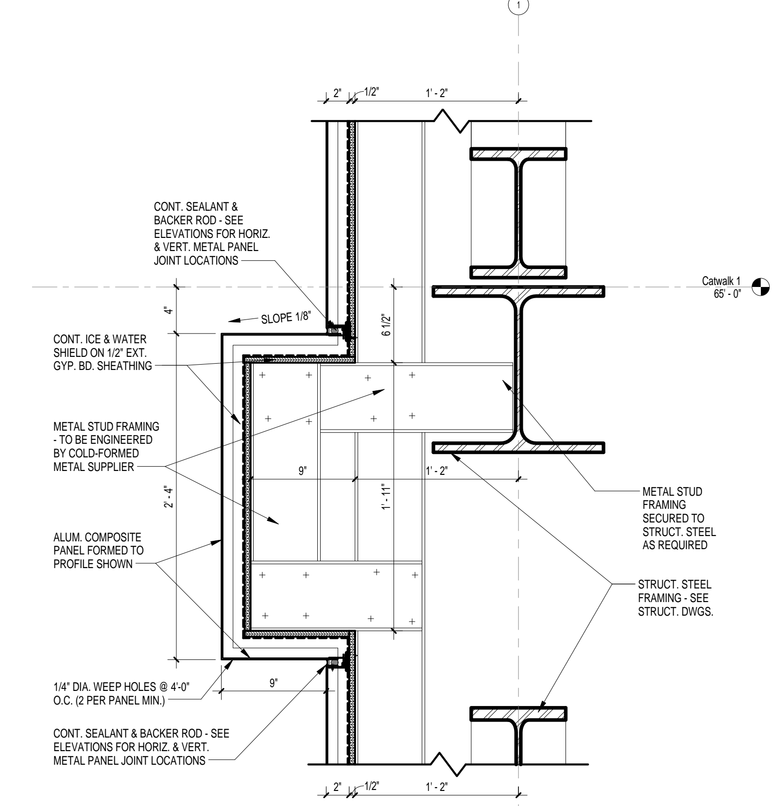
2 SECTION DETAIL A5.3 1 1/2" = 1'-0" REFERENCED ON: A5.2
