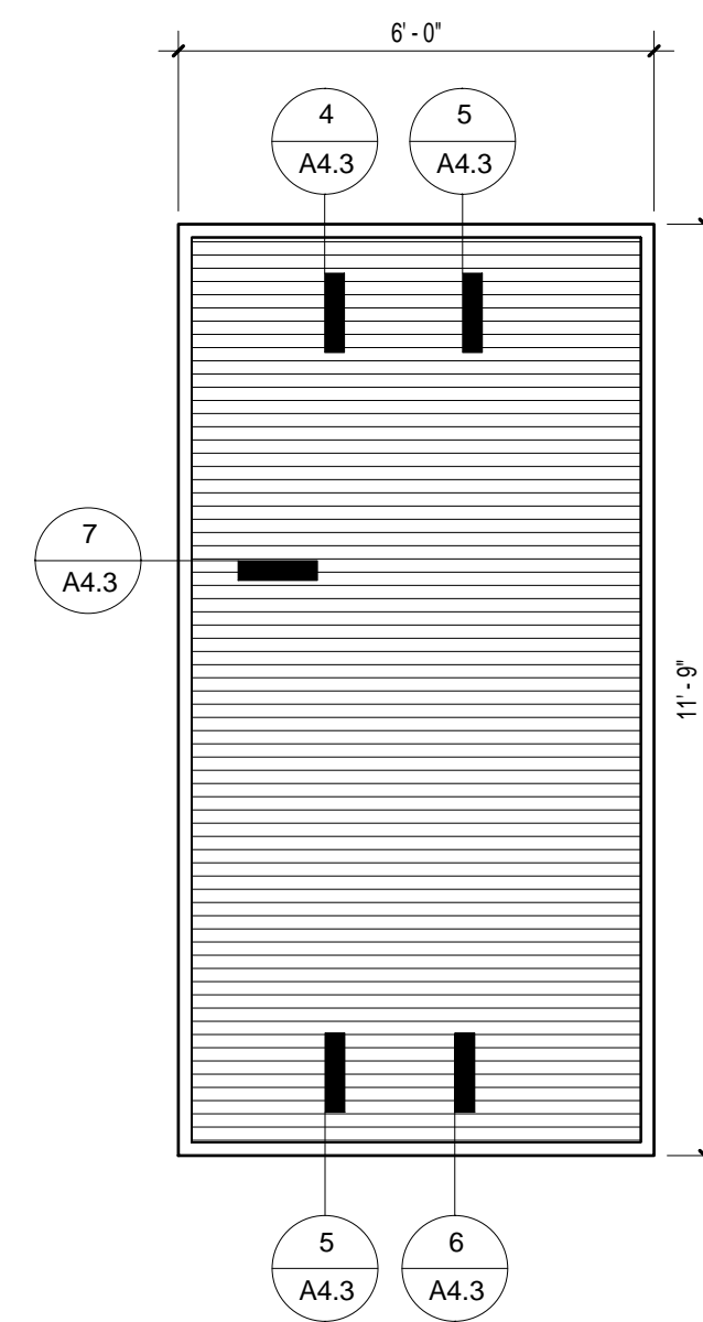
LOUVER L1 EXTERIOR ALUMINUM
