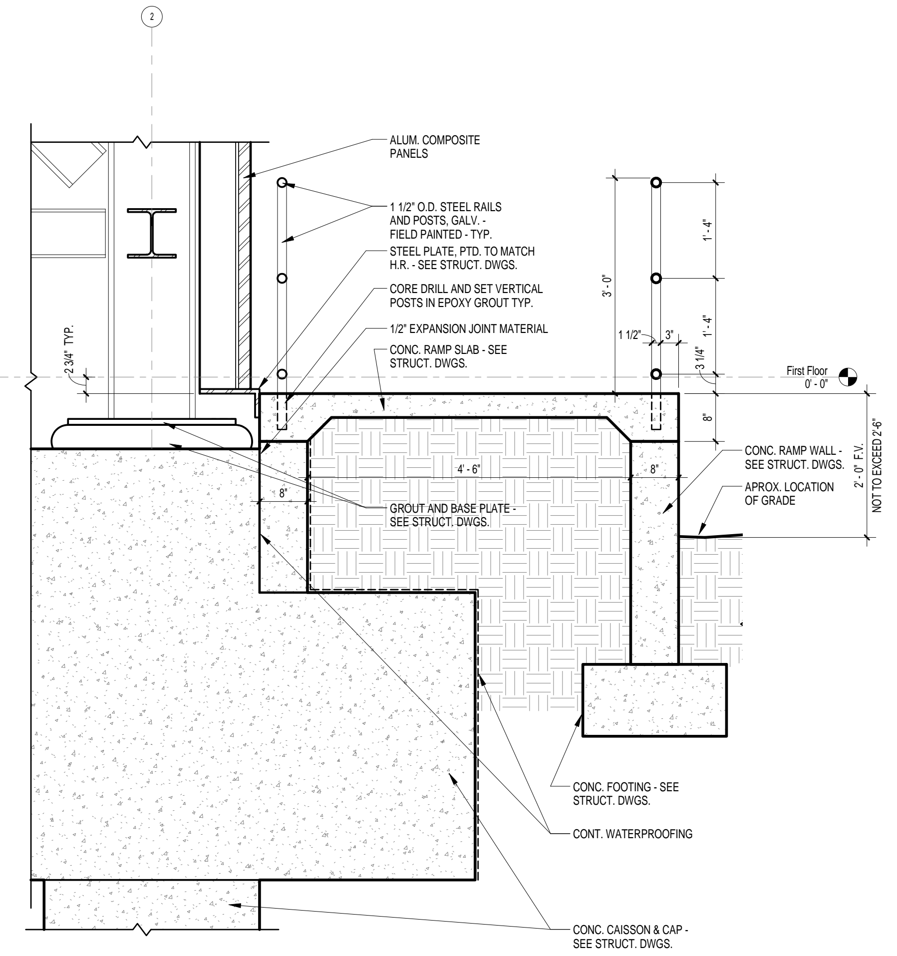
1 RAMP SECTION 1 A6.1 3/4" = 1'-0" REFERENCED ON: A1.1
