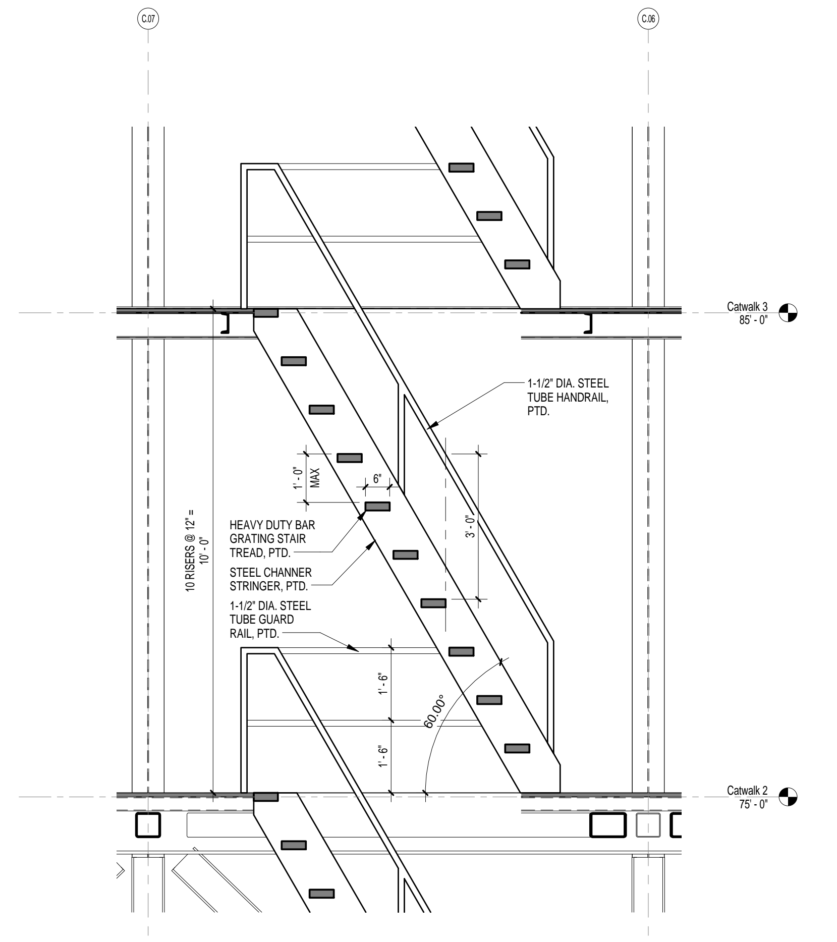
3 SHIPS LADDER SECTION A6.1 1/2" = 1'-0" REFERENCED ON: A5.1
