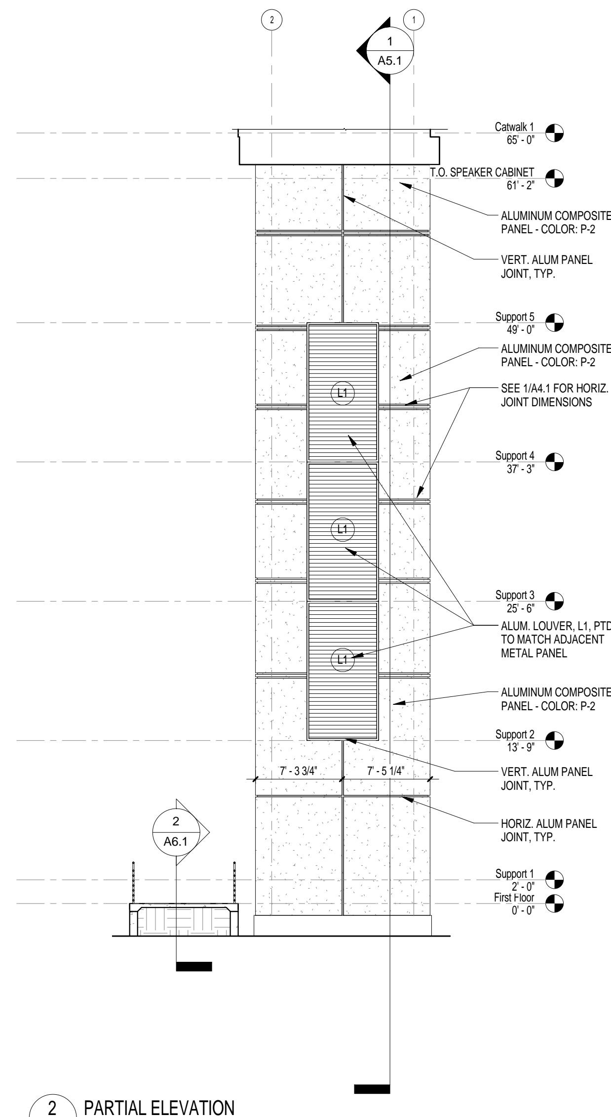
2 PARTIAL ELEVATION A4.3 1/8" = 1'-0" REFERENCED ON: A1.1
