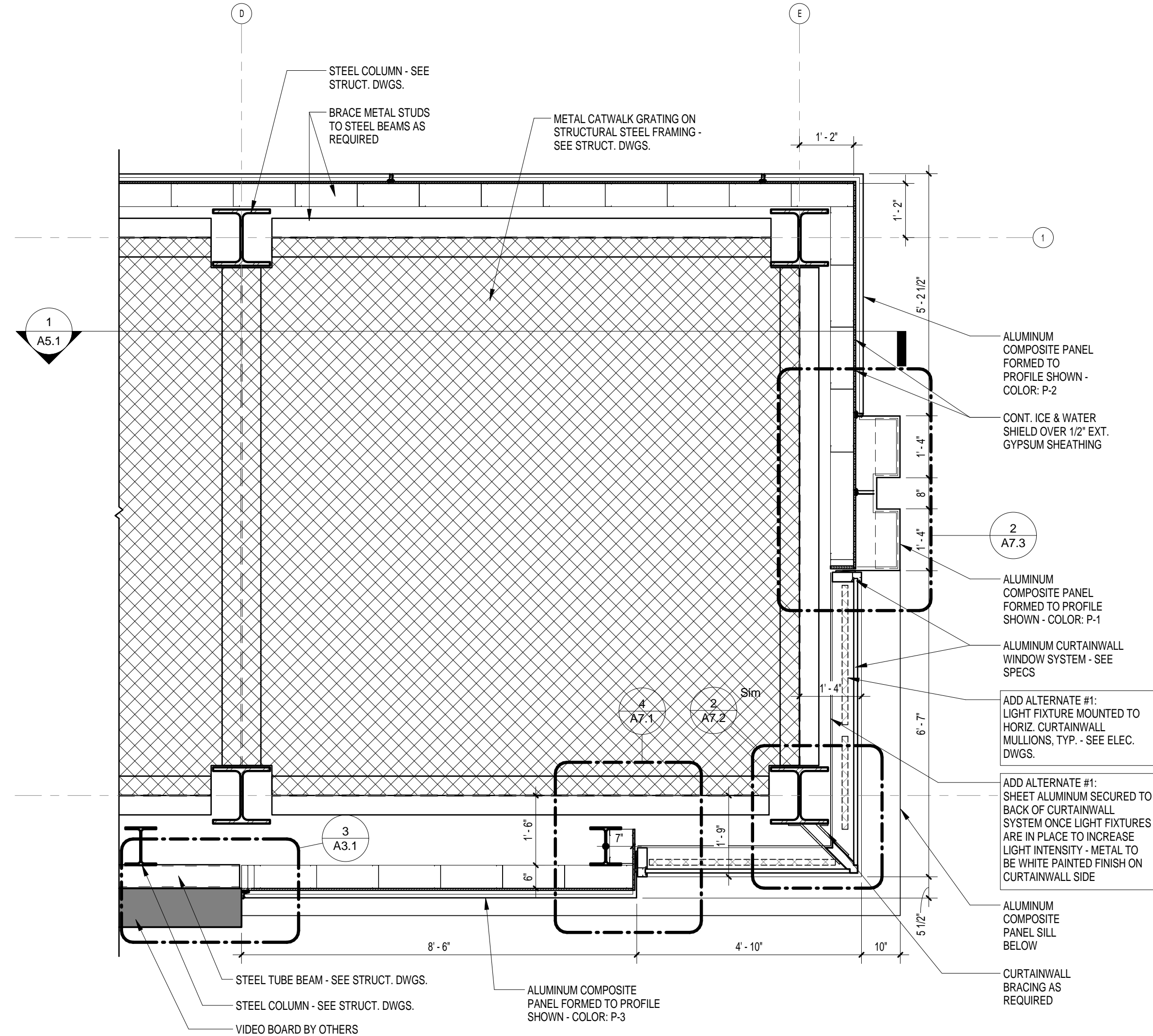
1 ENLARGED PLAN A3.1 1/2" = 1'-0" REFERENCED ON: A1.1
