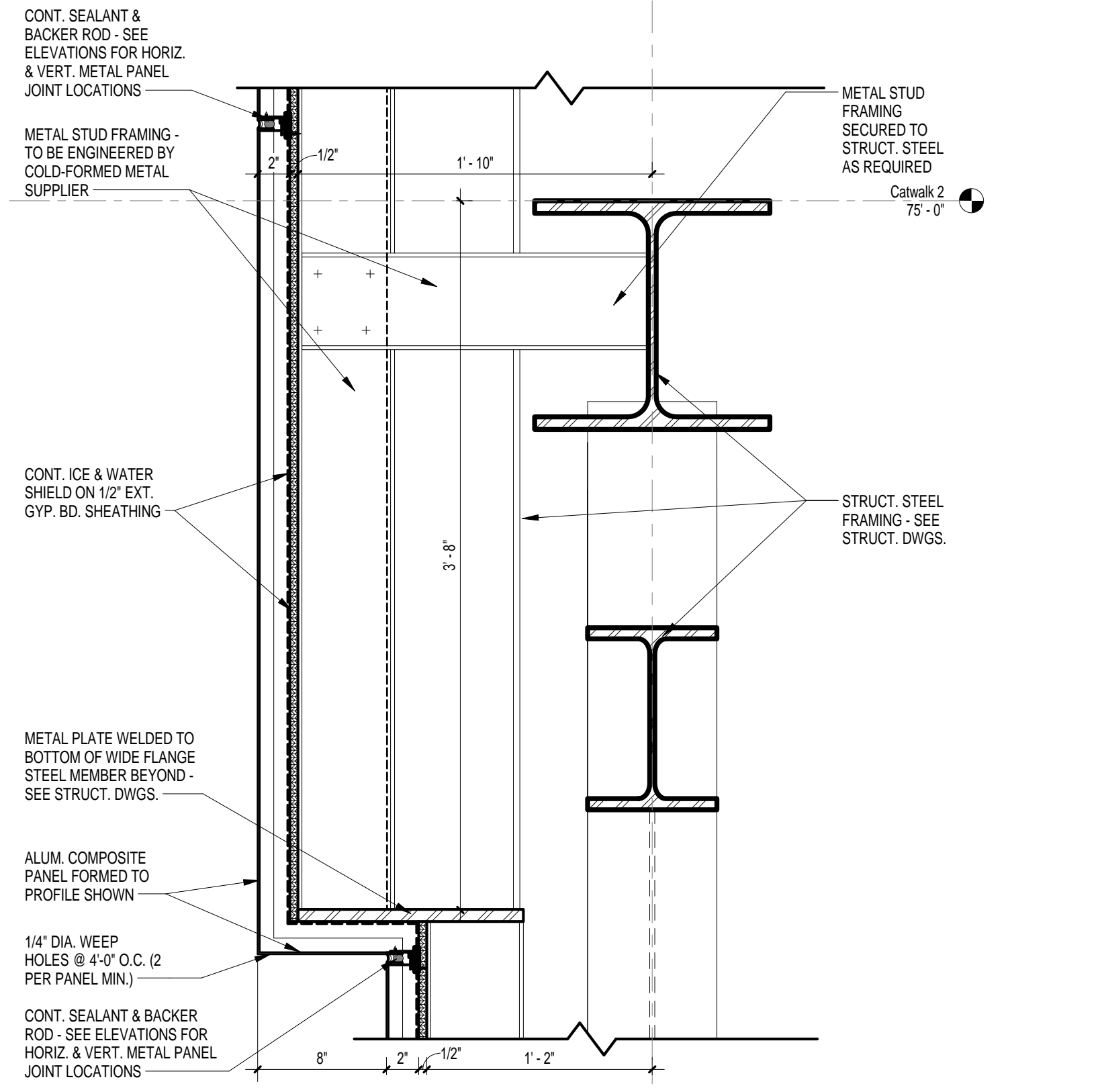
3 SECTION DETAIL A5.4 1 1/2" = 1'-0" REFERENCED ON: A5.3
