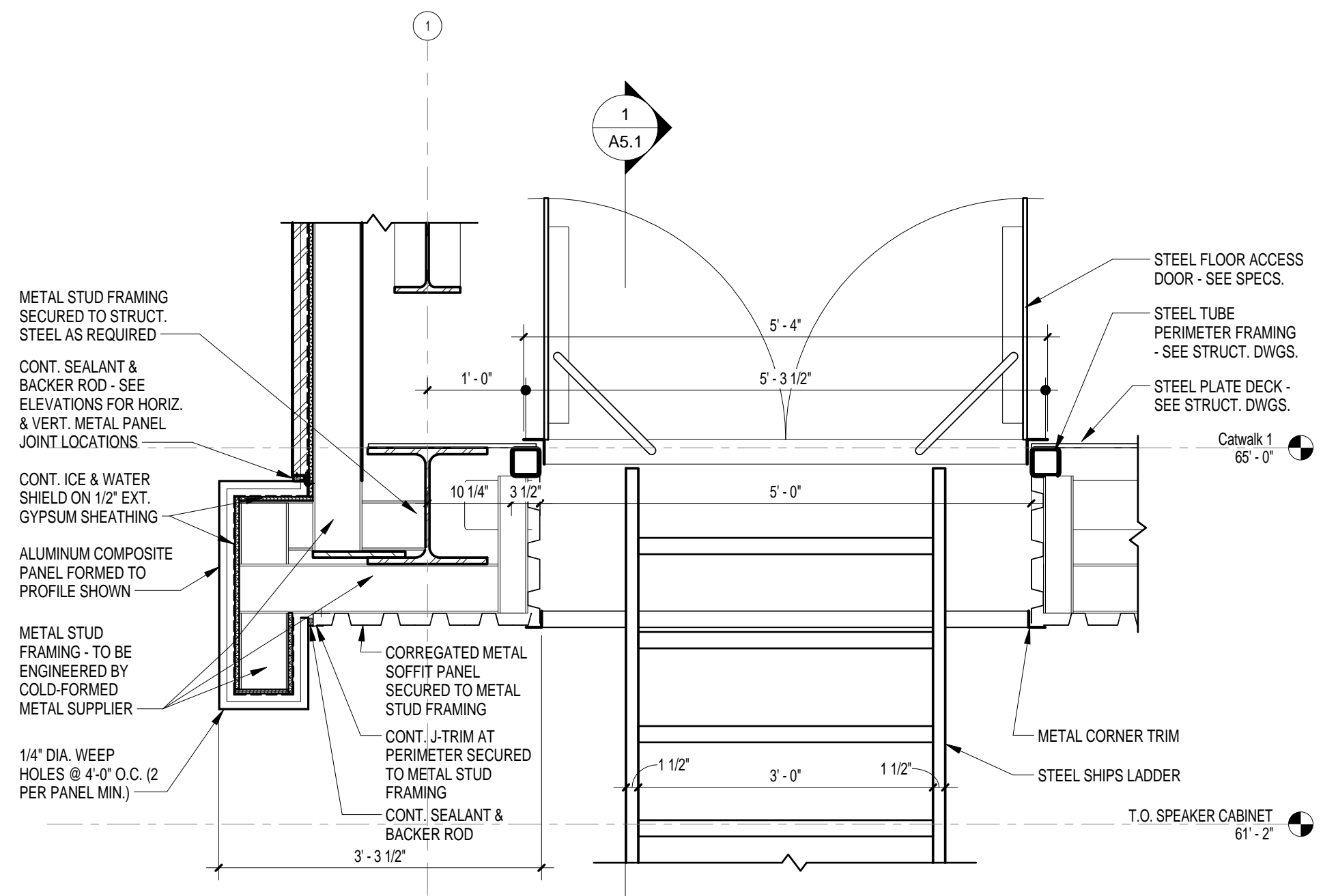
4 FLOOR ACCESS DOOR SECTION A6.1 3/4" = 1'-0" REFERENCED ON: A1.1
