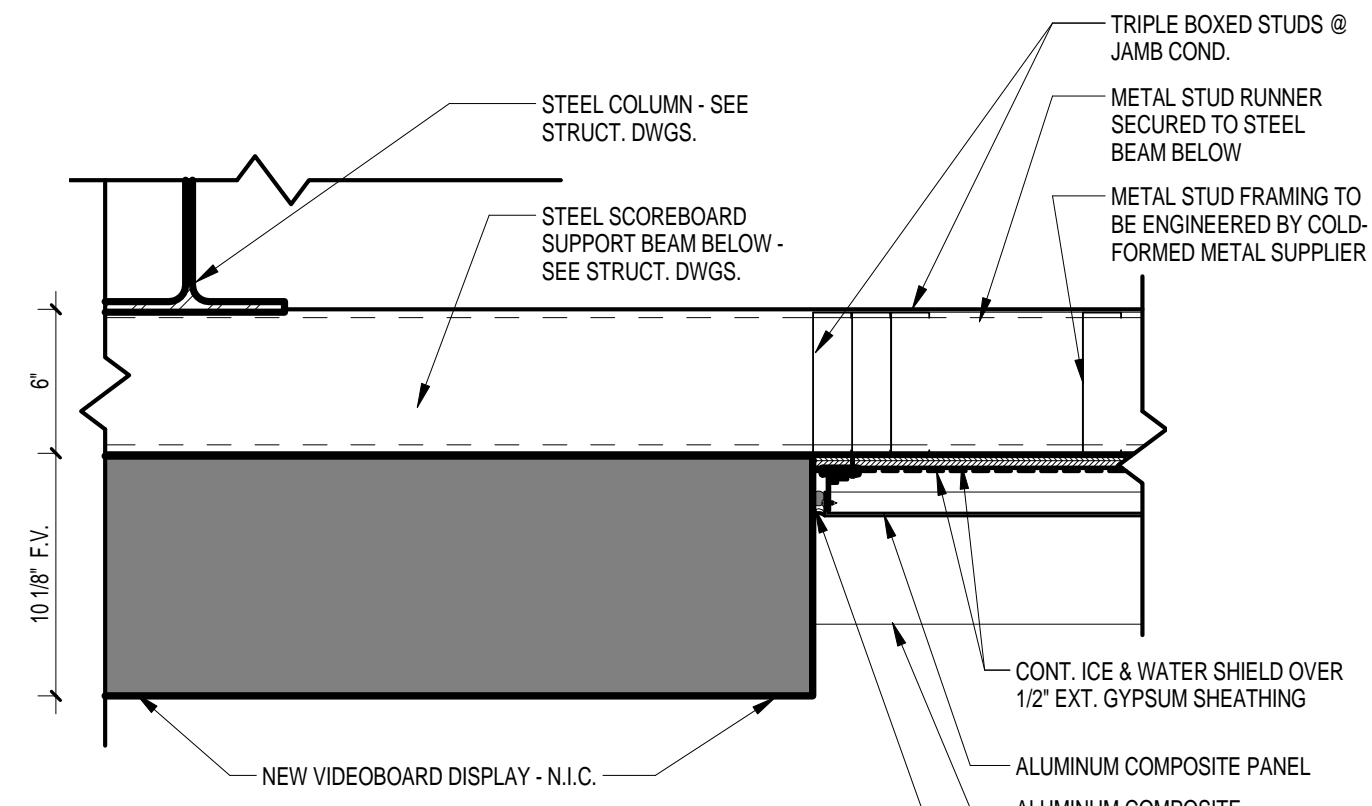
3 PLAN DETAIL A3.1 1/2" = 1'-0" REFERENCED ON: A3.1
