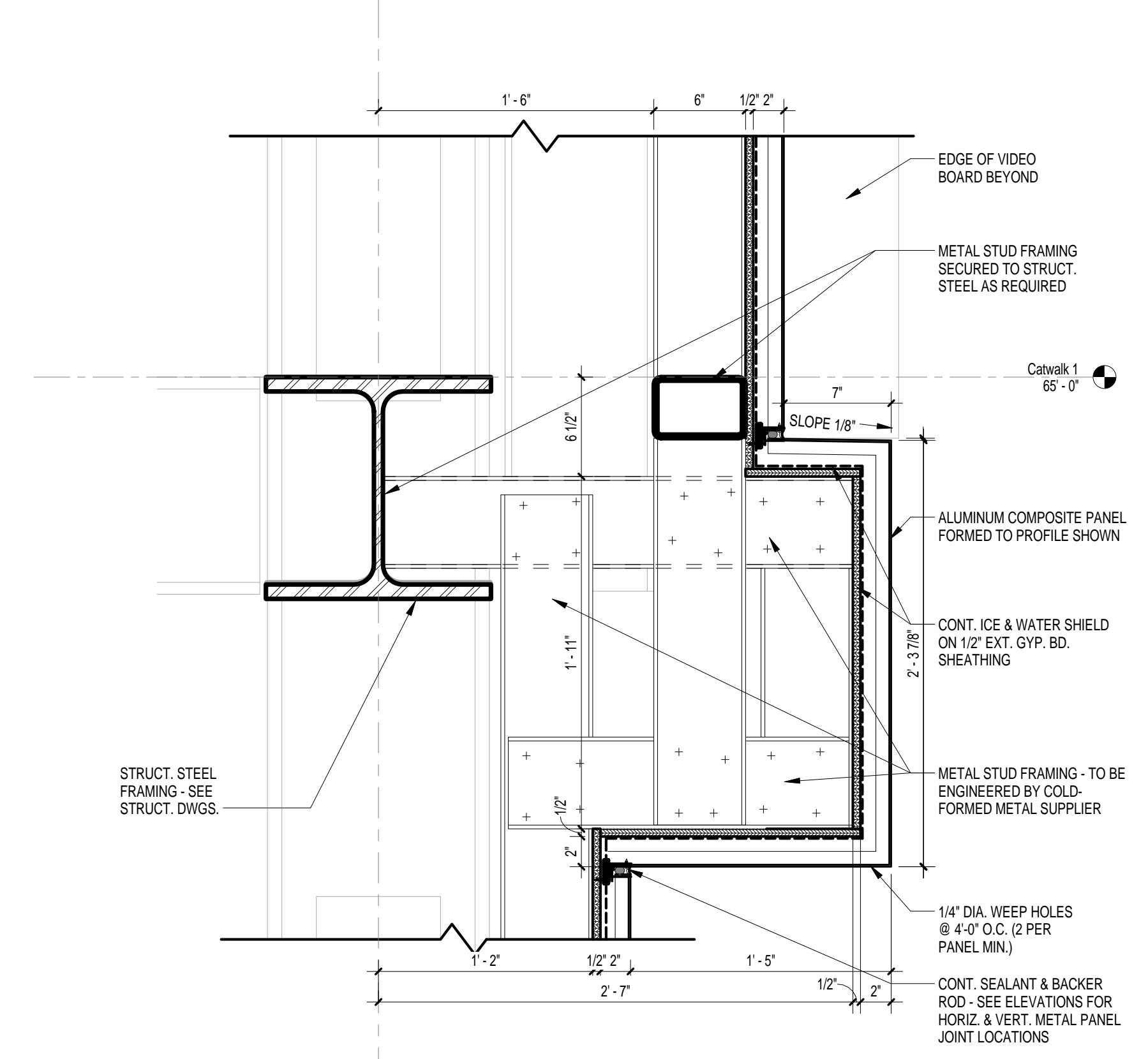
3 SECTION DETAIL A5.3 1 1/2" = 1'-0" REFERENCED ON: A5.2
