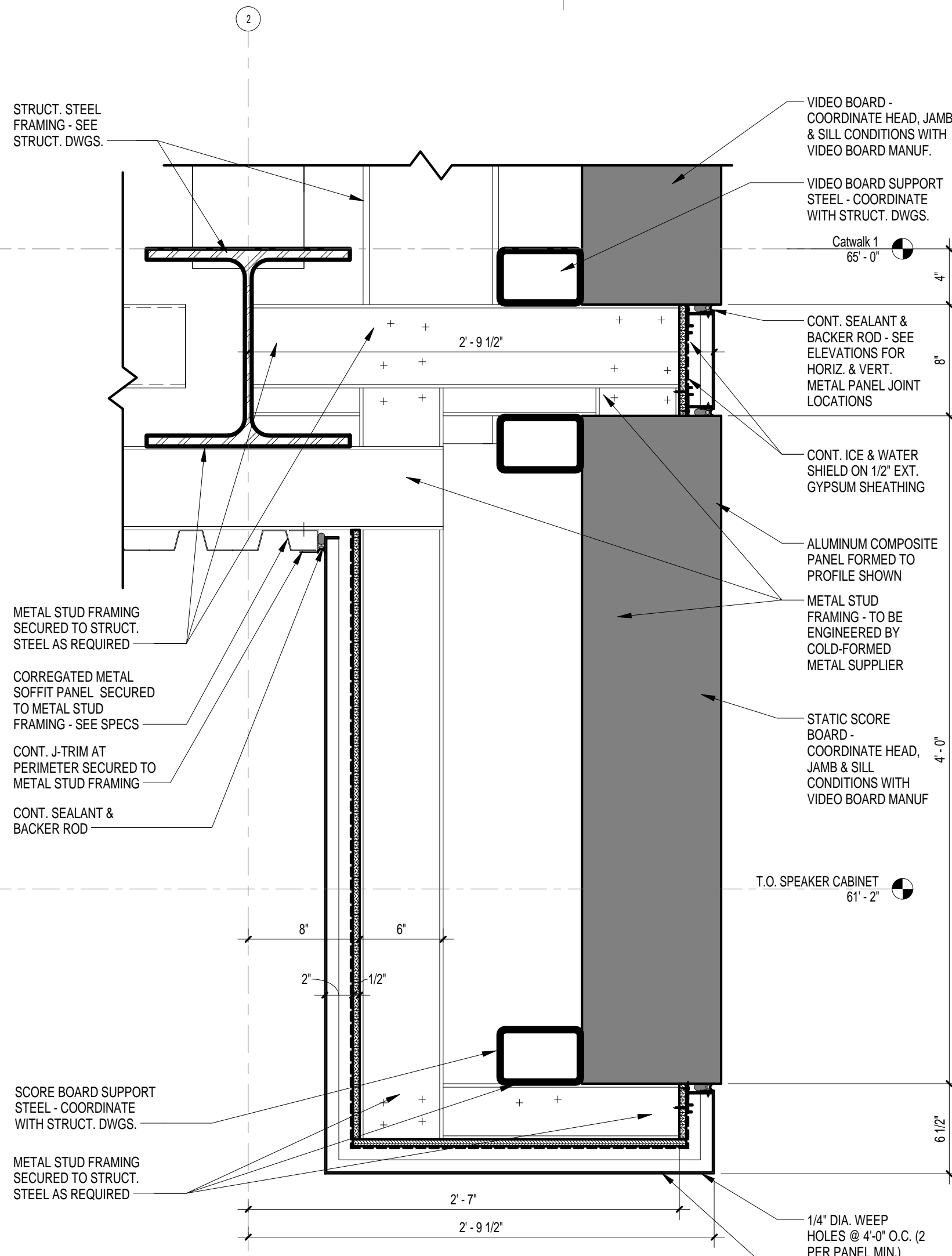
4 SECTION DETAIL A5.4 1 1/2" = 1'-0" REFERENCED ON: A5.3
