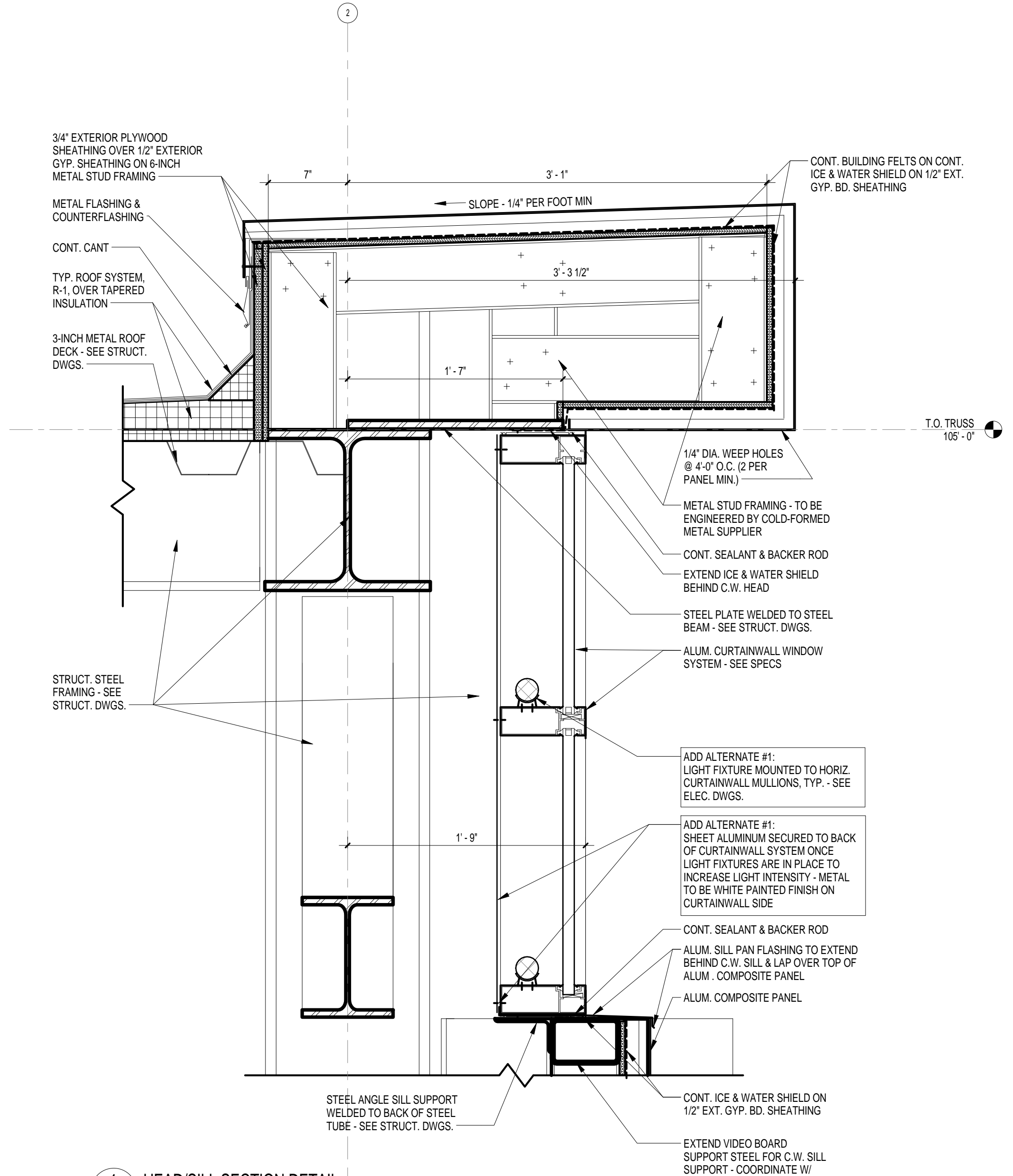
1 HEAD/SILL SECTION DETAIL A7.4 1 1/2" = 1'-0" REFERENCED ON: A5.2
