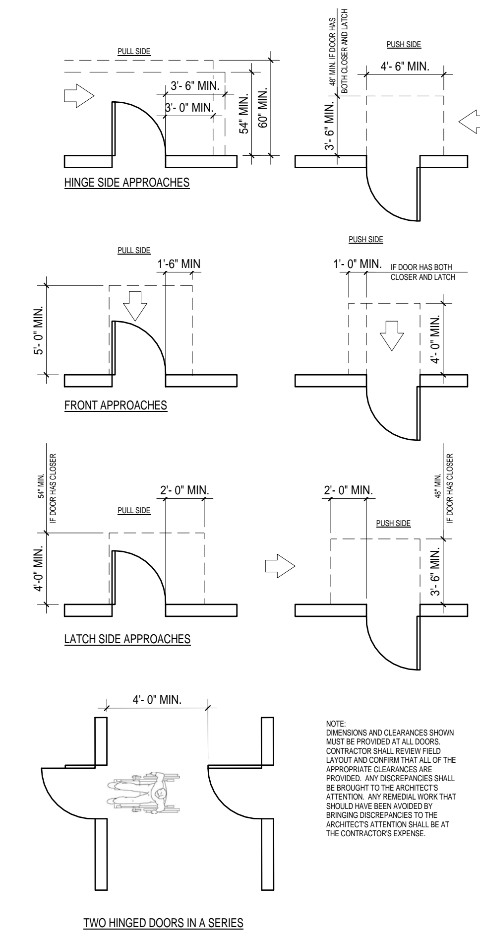
ANSI 117.1 - MANEUVERING CLEARANCES
