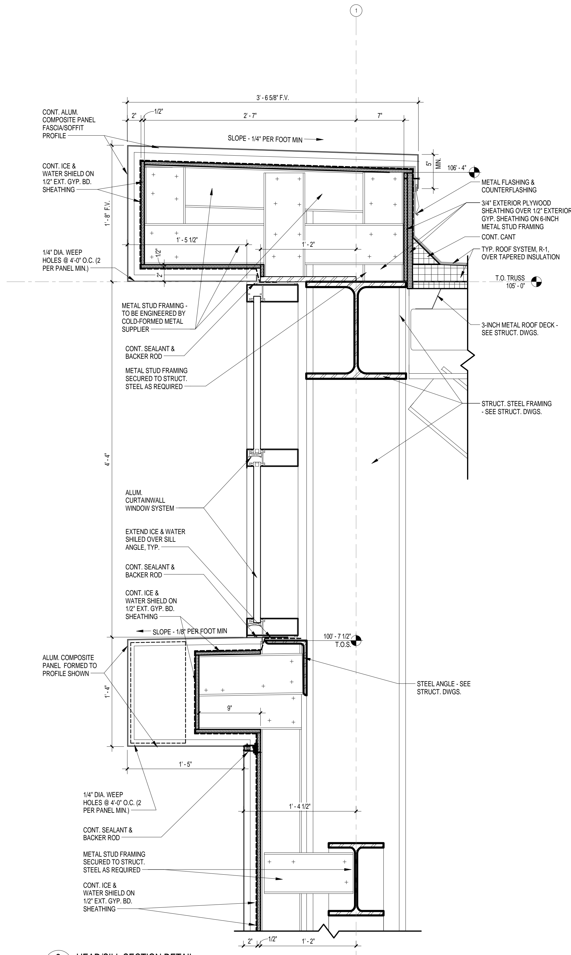
2 HEAD/SILL SECTION DETAIL A7.4 1 1/2" = 1'-0" REFERENCED ON: A5.2
