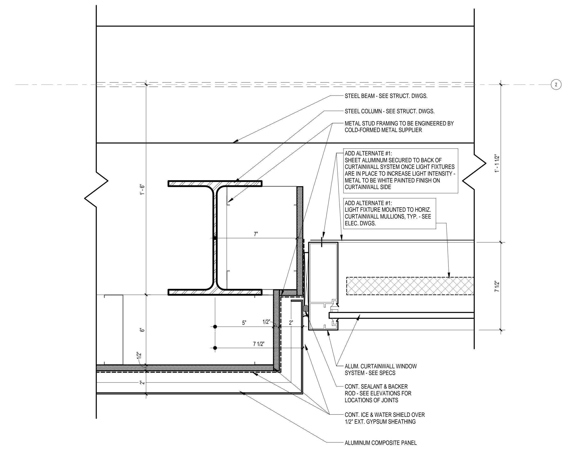
4 JAMB PLAN DETAIL A7.1 3" = 1'-0" REFERENCED ON: A3.1
