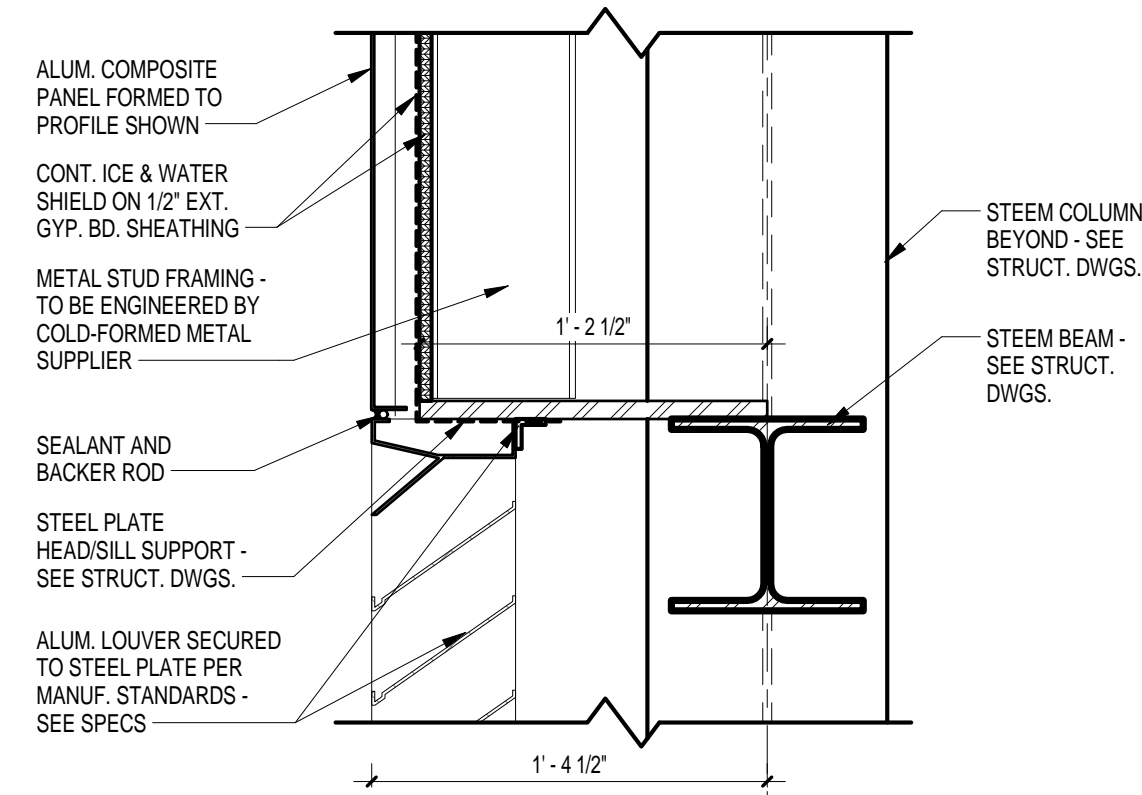
4 LOUVER HEAD SECTION DETAIL A4.3 1 1/2" = 1'-0" REFERENCED ON: A4.3
