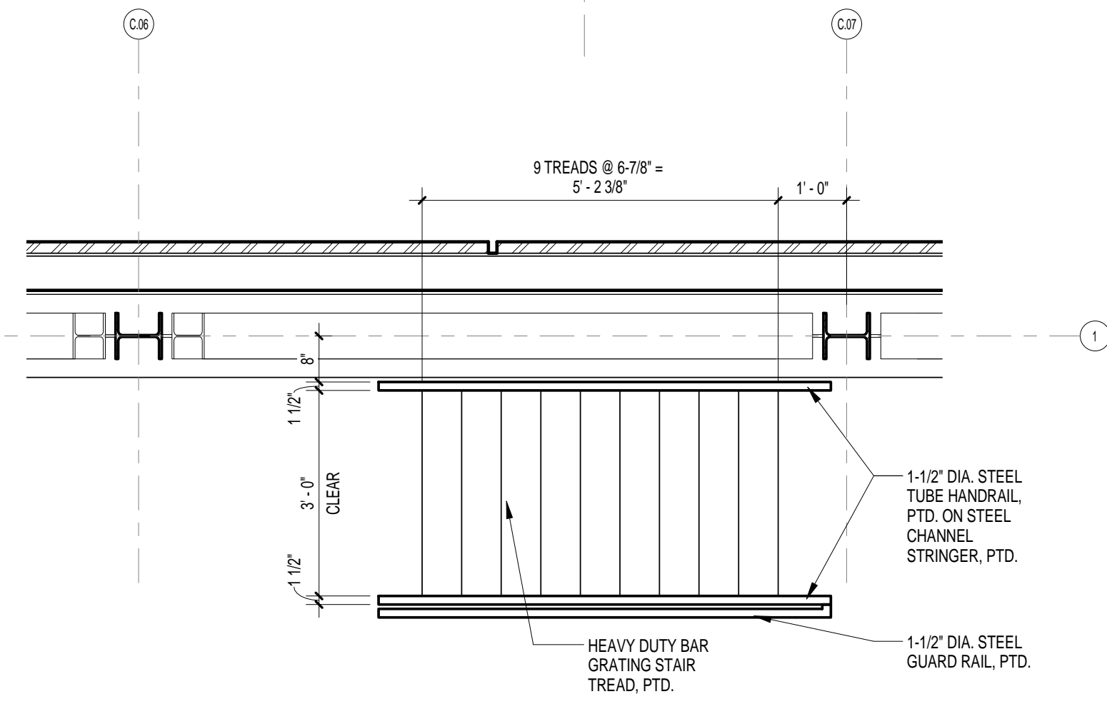
4 ENLARGED PLAN @ SHIPS LADDER A3.1 1/2" = 1'-0" REFERENCED ON: A1.1
