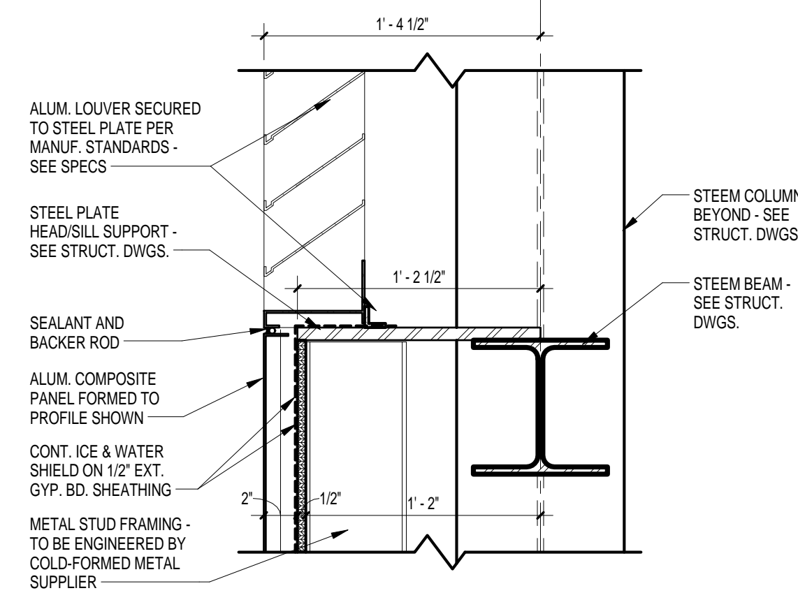
6 LOUVER SILL SECTION DETAIL A4.3 1 1/2" = 1'-0" REFERENCED ON: A4.3
