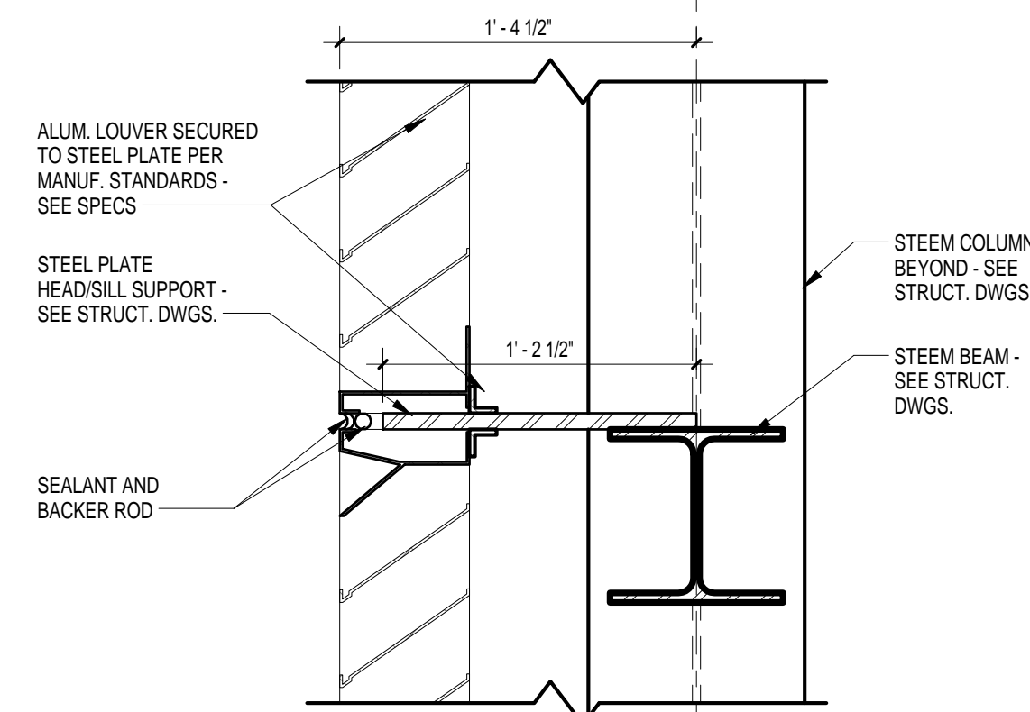
5 LOUVER HEAD/SILL SECTION DETAIL A4.3 1 1/2" = 1'-0" REFERENCED ON: A4.3
