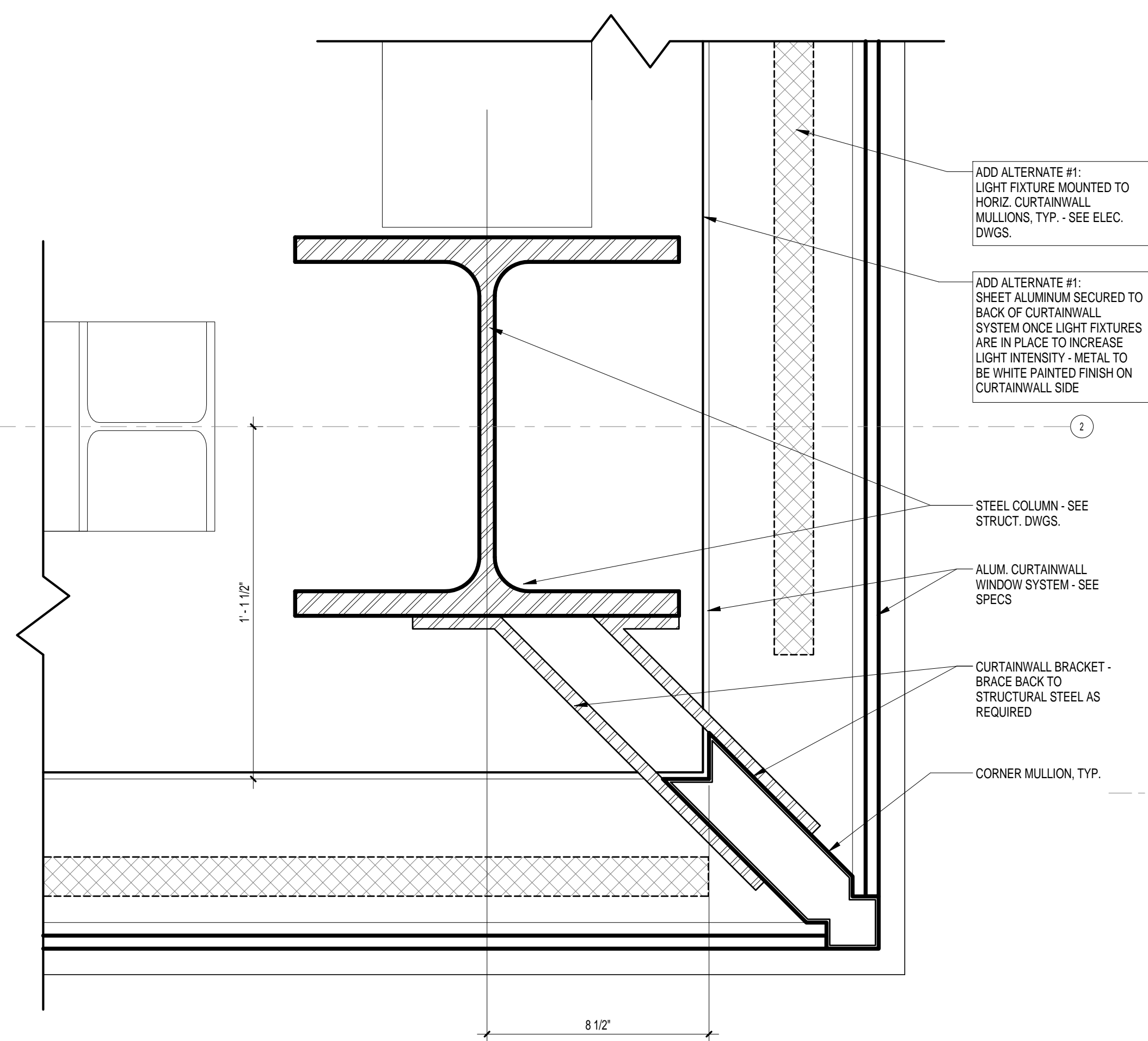
2 JAMB PLAN DETAIL A7.2 3" = 1'-0" REFERENCED ON: A1.2
