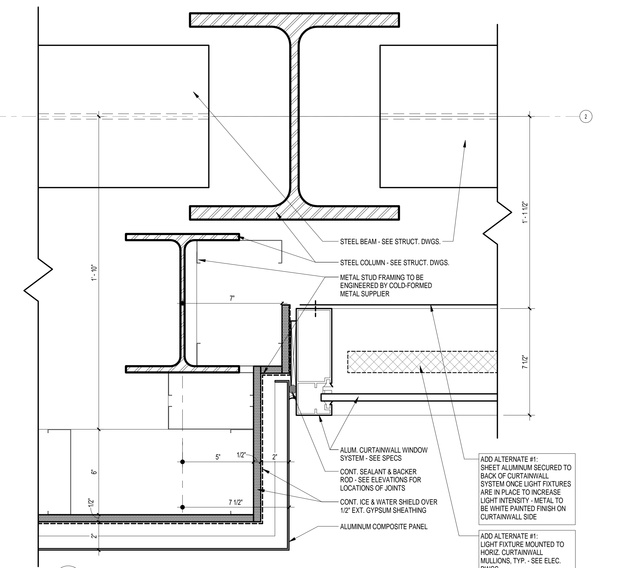
3 JAMB PLAN DETAIL A7.2 3" = 1'-0" REFERENCED ON: A1.2
