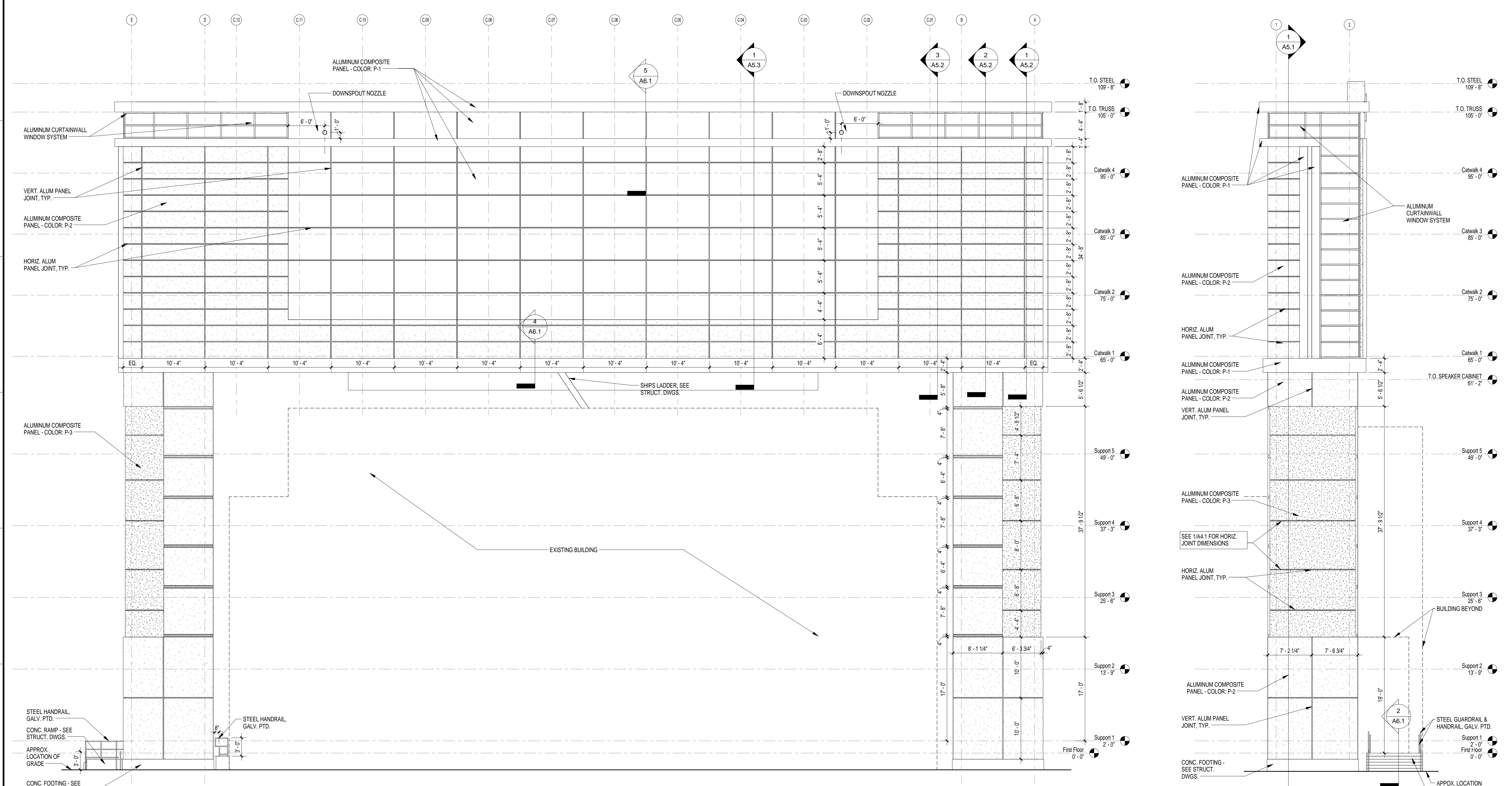
1 NORTH ELEVATION A4.1 1/8" = 1'-0" REFERENCED ON: A1.1
