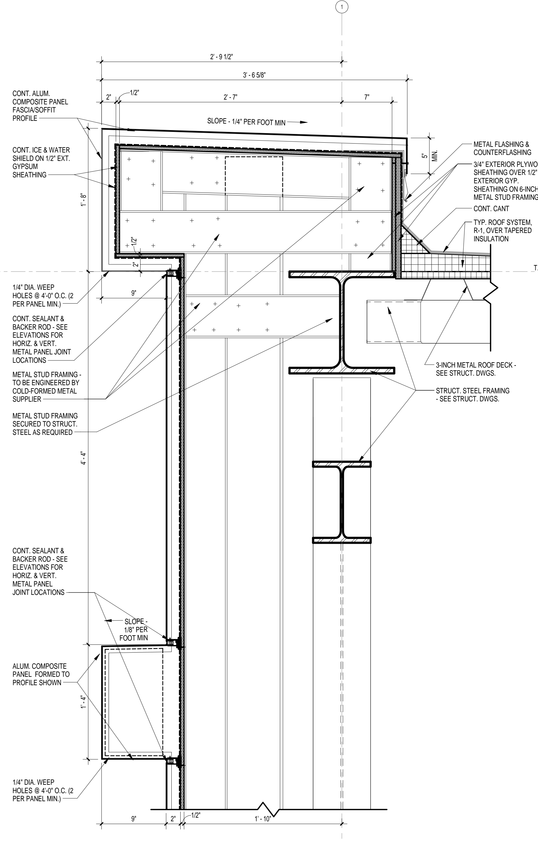
2 SECTION DETAIL A5.4 1 1/2" = 1'-0" REFERENCED ON: A5.3
